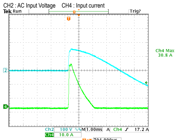
INPUT=115VAC/50HZ @ FULL LOAD
